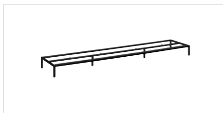
optionales Metallgestell 9966 B/H/T 180/13/39,5
